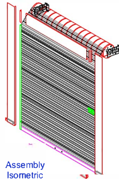
Assembly Isometric
