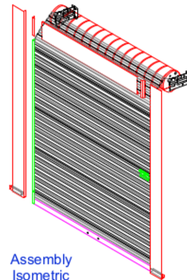
Assembly Isometric
